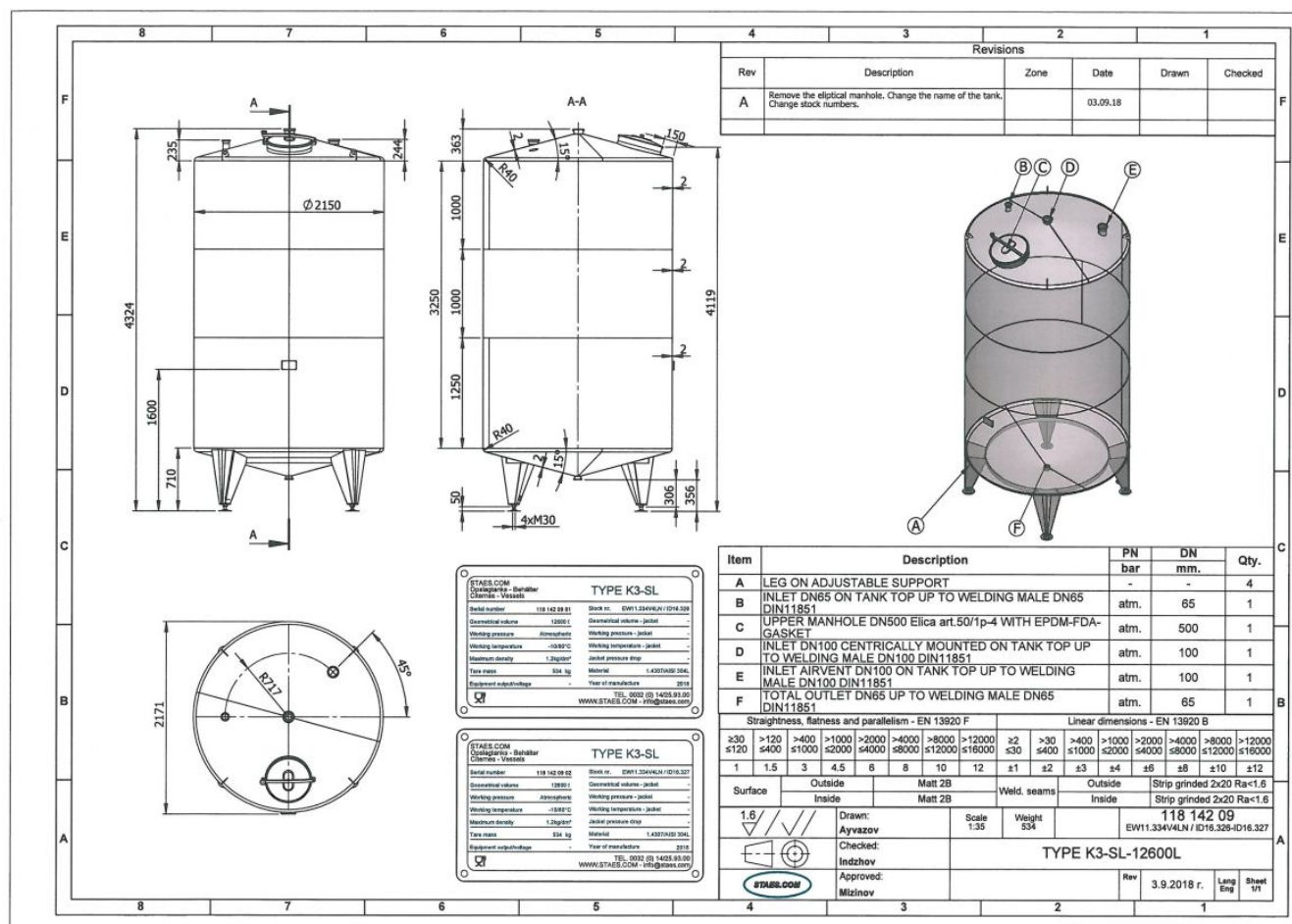
Technical drawing
