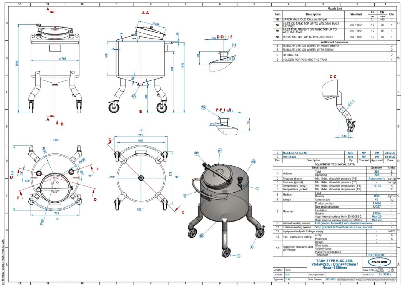
Technical drawing
