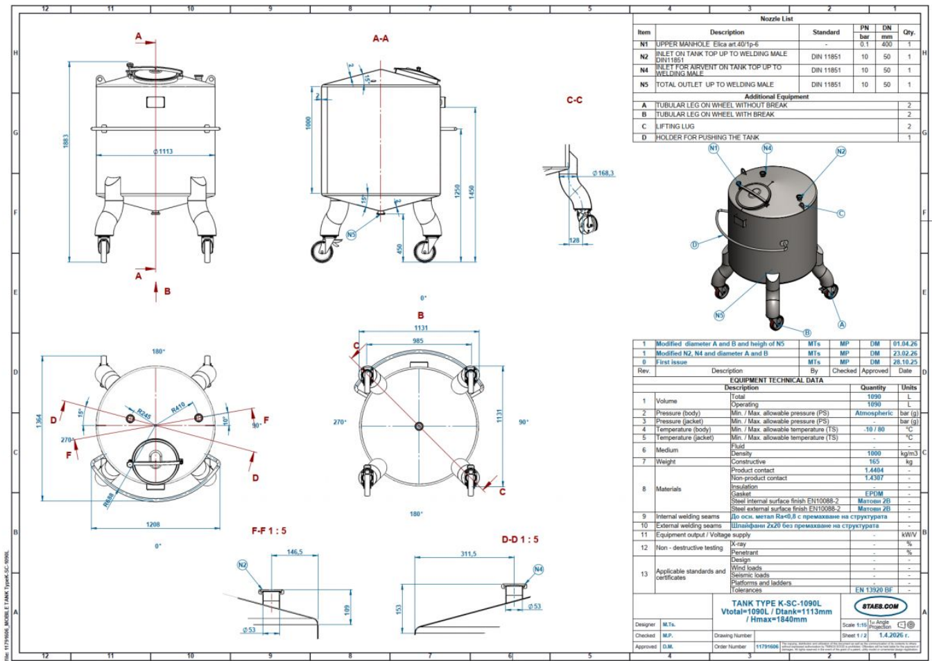
Technical drawing
