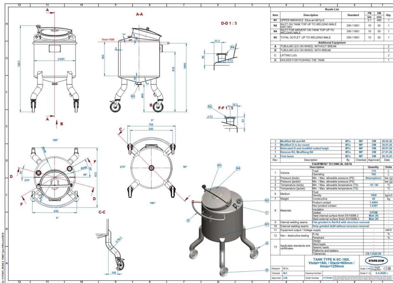
Technical drawing
