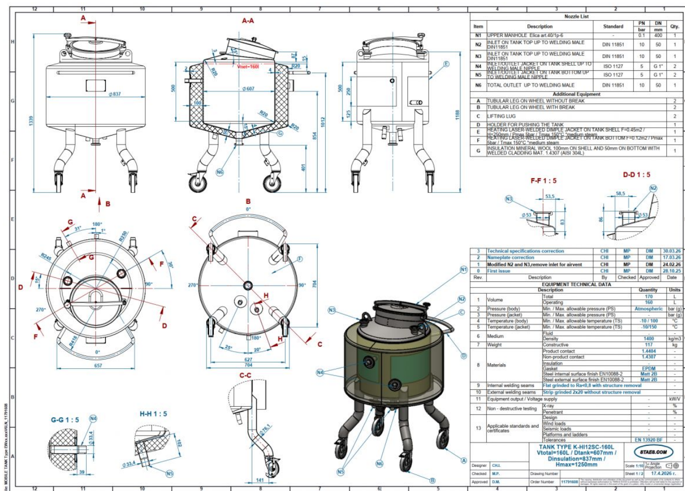
Technical drawing
